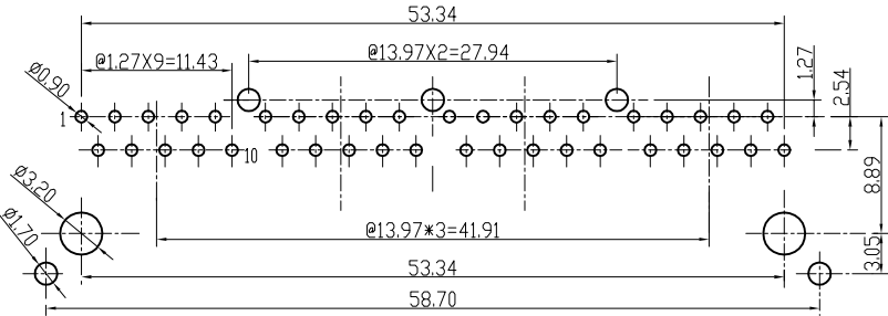
PC BOARD LAYOUT THICKNESS=1.6mm
